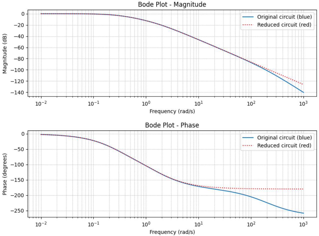
Figure 41: Bode Plots
