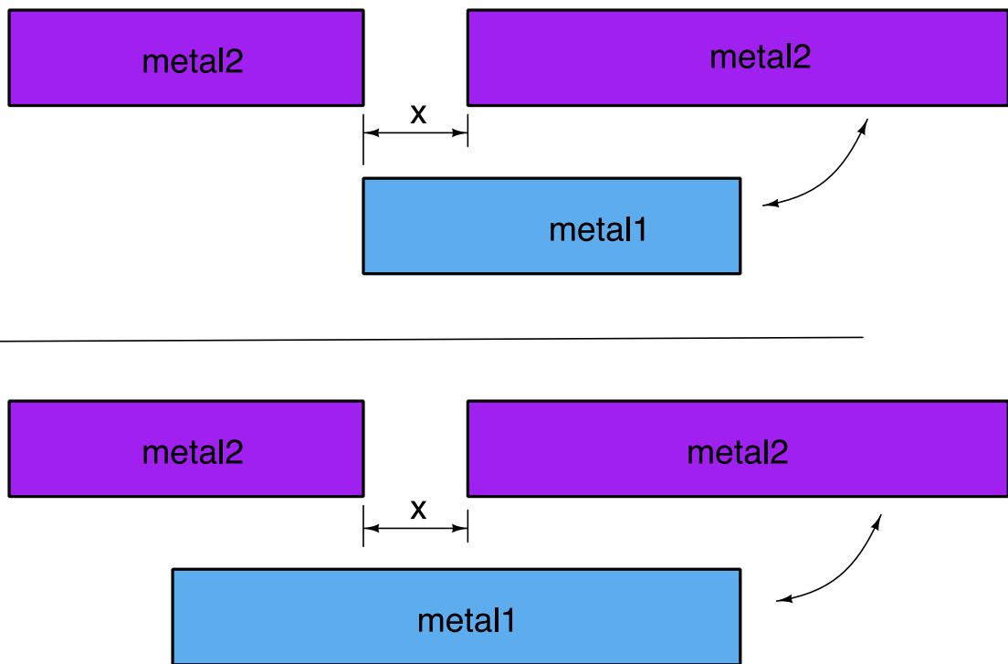
Figure 19: Lateral fringe shielding (2/2)
