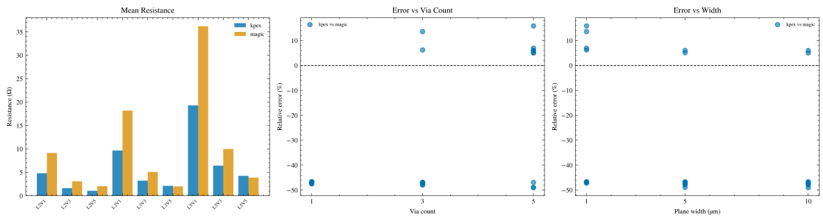
sky130 — Resistance Comparison
