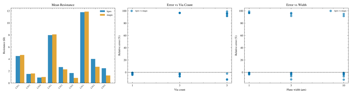
sky130 — Resistance Comparison
