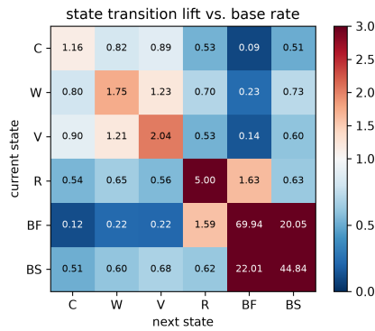
Fig. 3. Heatmap displaying the transition lifts between each observable state.
