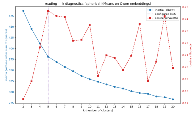
Fig. 1. Reading elbow plot
