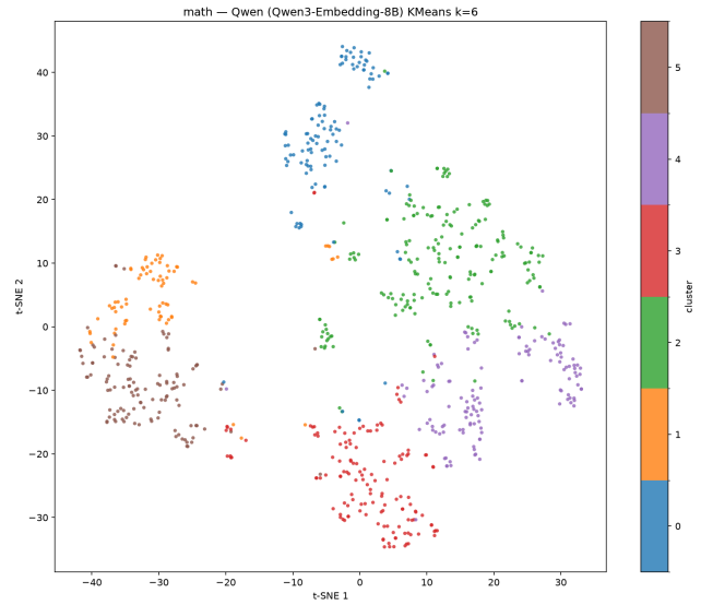
Fig. 2. Mathematics t-SNE plot. Each dot represents a question, and the cluster key shown on the side corresponds to the clusters described in Table II.
