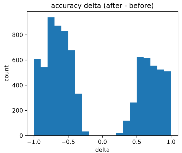
Fig. 5. Histogram displaying the distribution of change in response accuracy following changepoints
