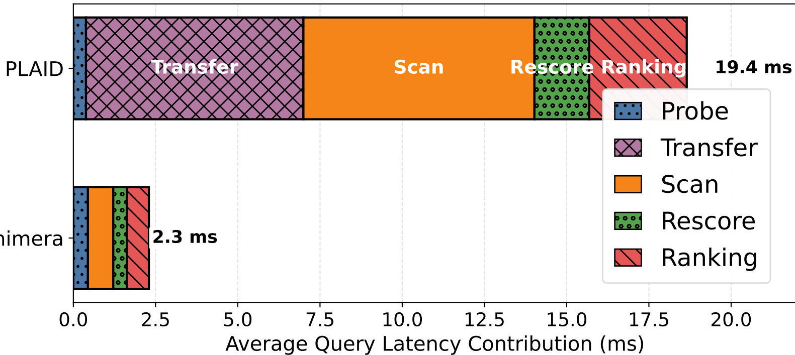
LoTTE: PLAID vs Chimera (Recall@100 = 0.9)
