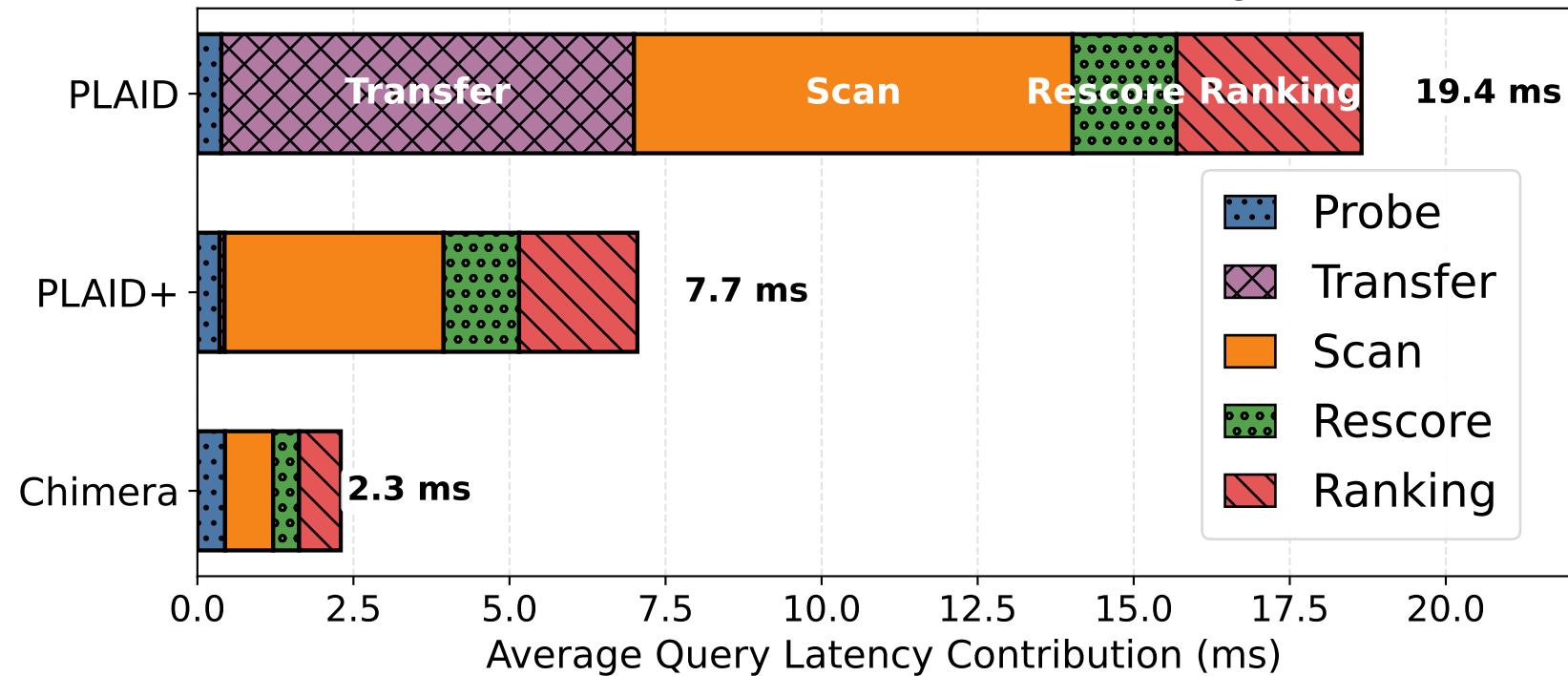
LoTTE: PLAID vs PLAID+ vs Chimera (Recall@100 = 0.9)
