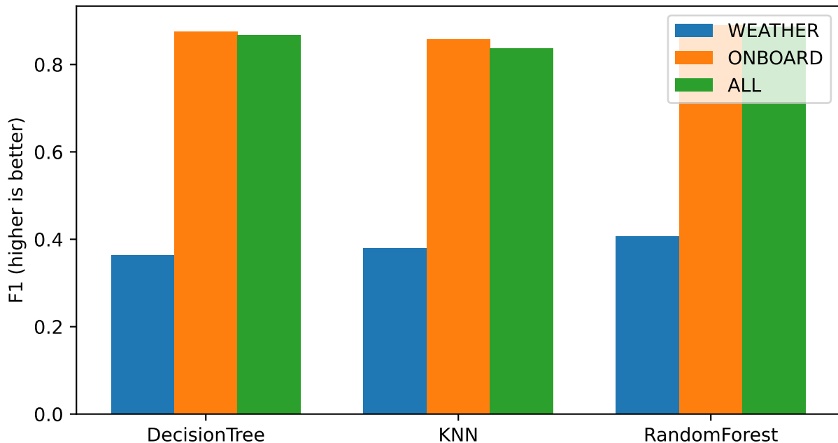
High-deviation classification F1 by model and feature set
