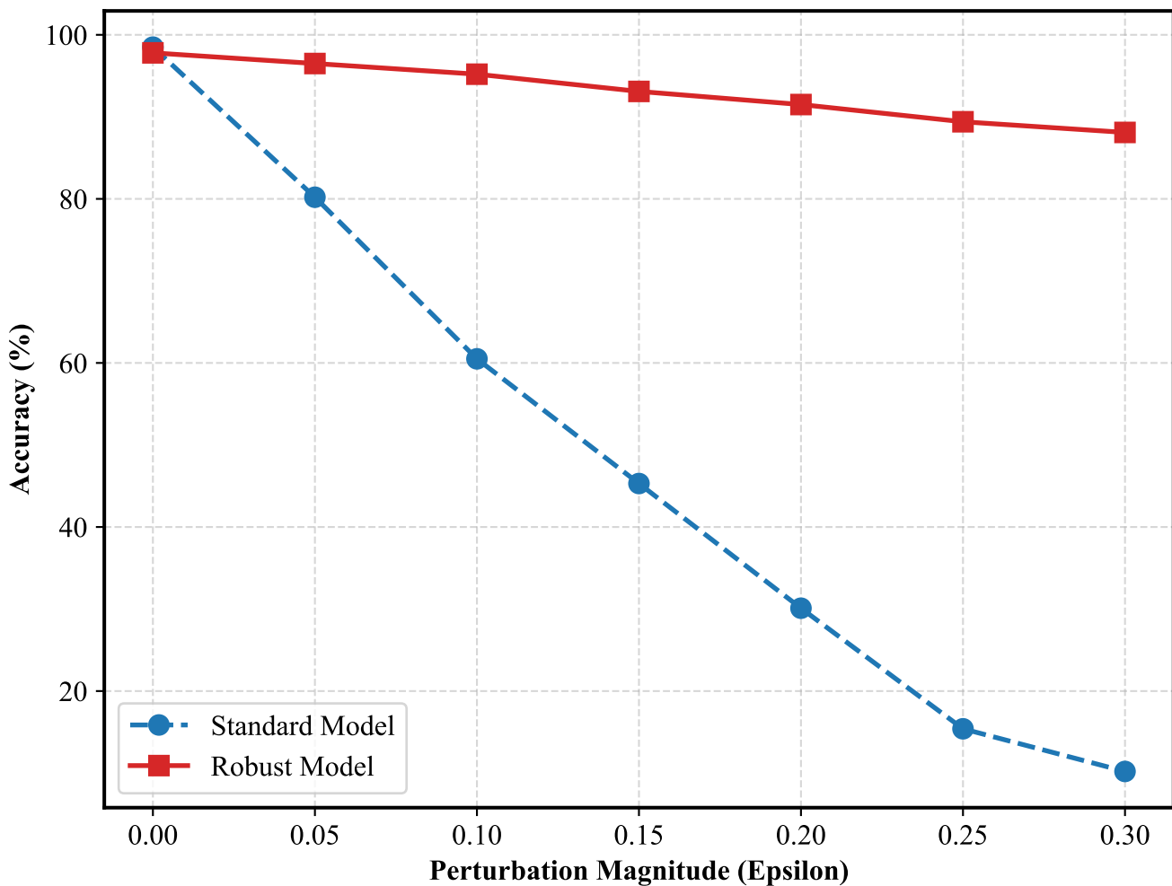
Robustness Evaluation under FGSM Attack
