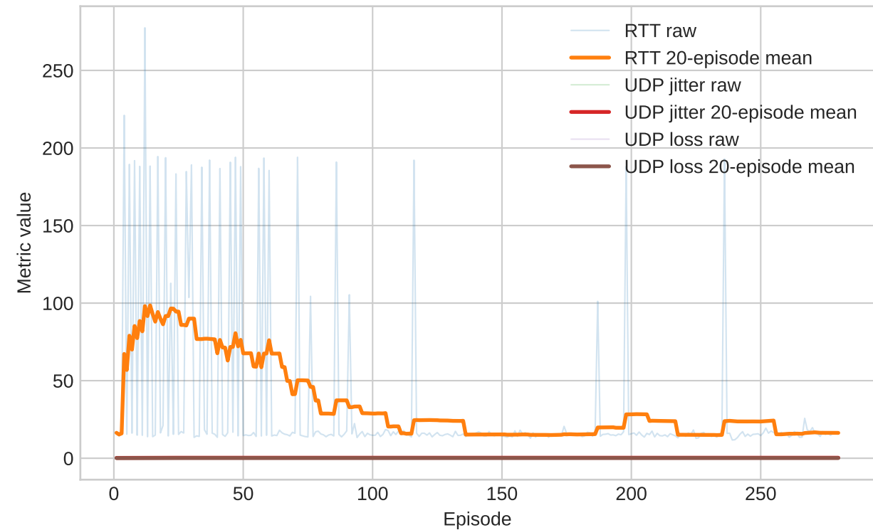
Delay, Jitter, and Loss
