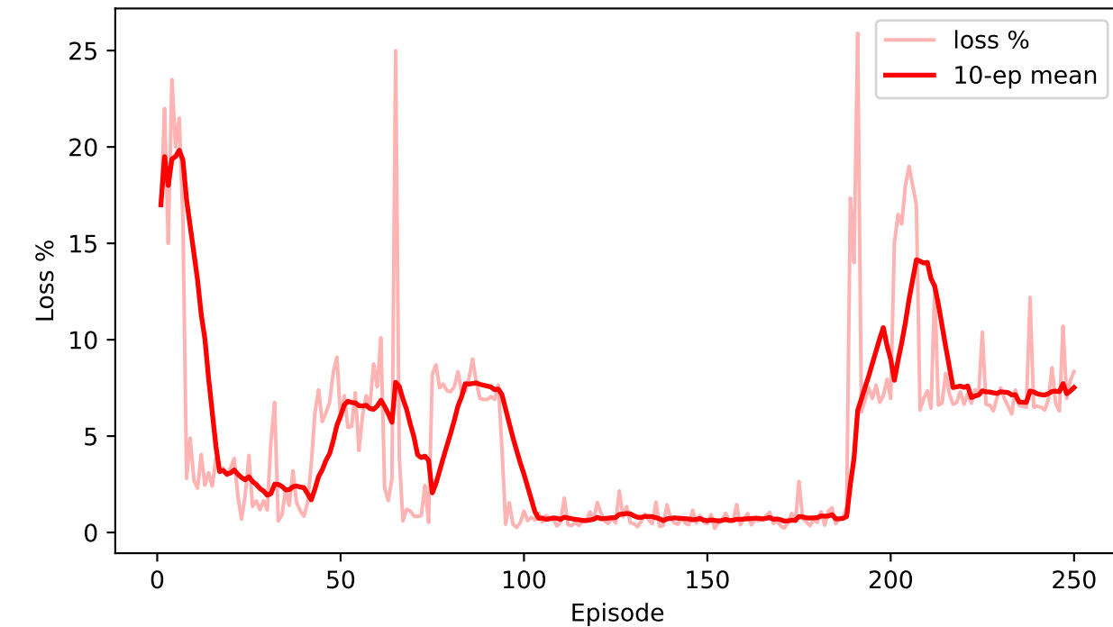
UDP Packet Loss per Episode
