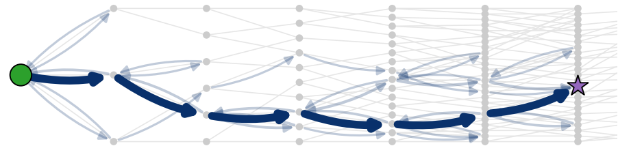
b CoNet, single-attempt training: p = 0.993 , IPR = 1.10
