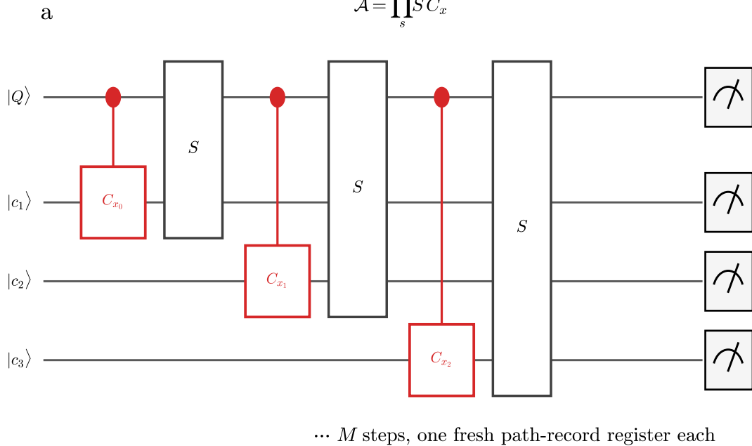
QuCoNet reasoning circuit:
