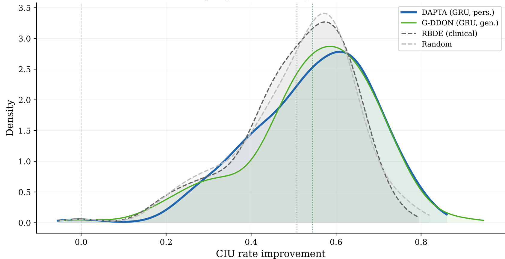
Distribution of per-patient CIU improvements (test set)
