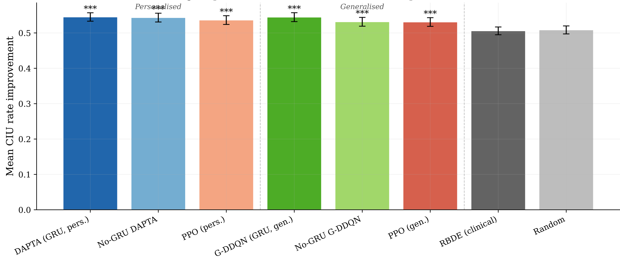
RQ2: Agent performance vs baselines (test set, * p < 0.05 vs RBDE)
