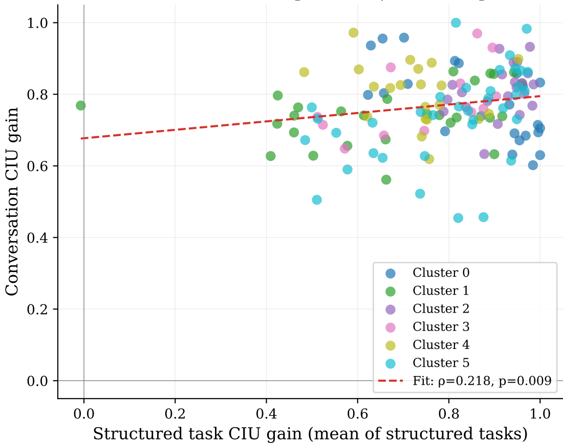
RQ3: Cross-task transfer (Spearman \rho = 0.218 , p = 0.009 )
