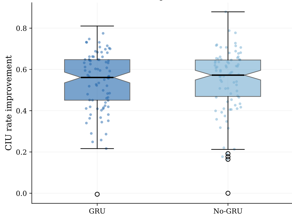
GRU benefit — Personalised (cluster-specific) (Wilcoxon p = 0.9401 )
