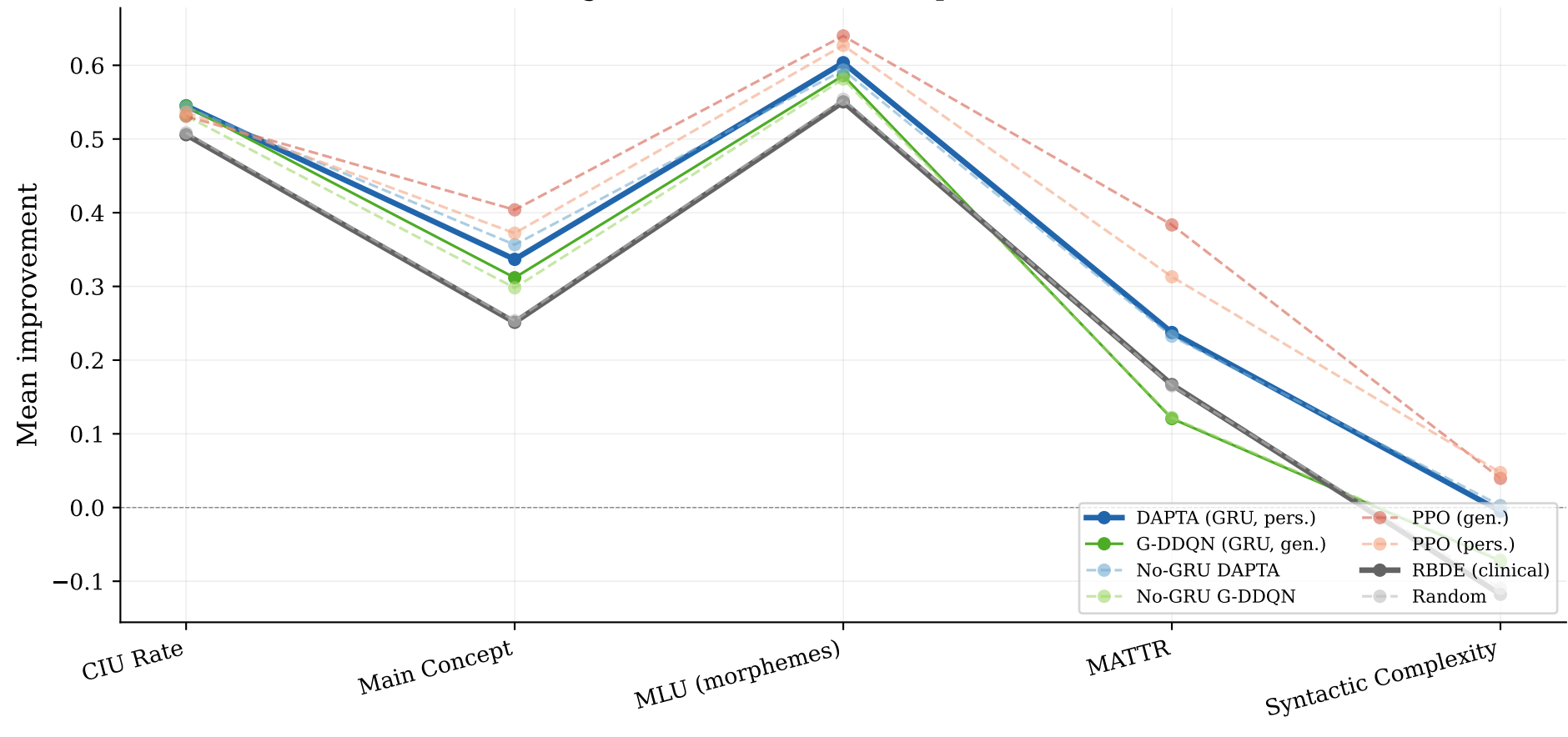
All agents: discourse metric profile (test set)
