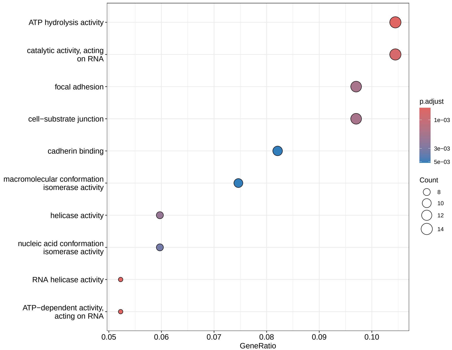
GO Enrichment: Translational Inhibitor 1
