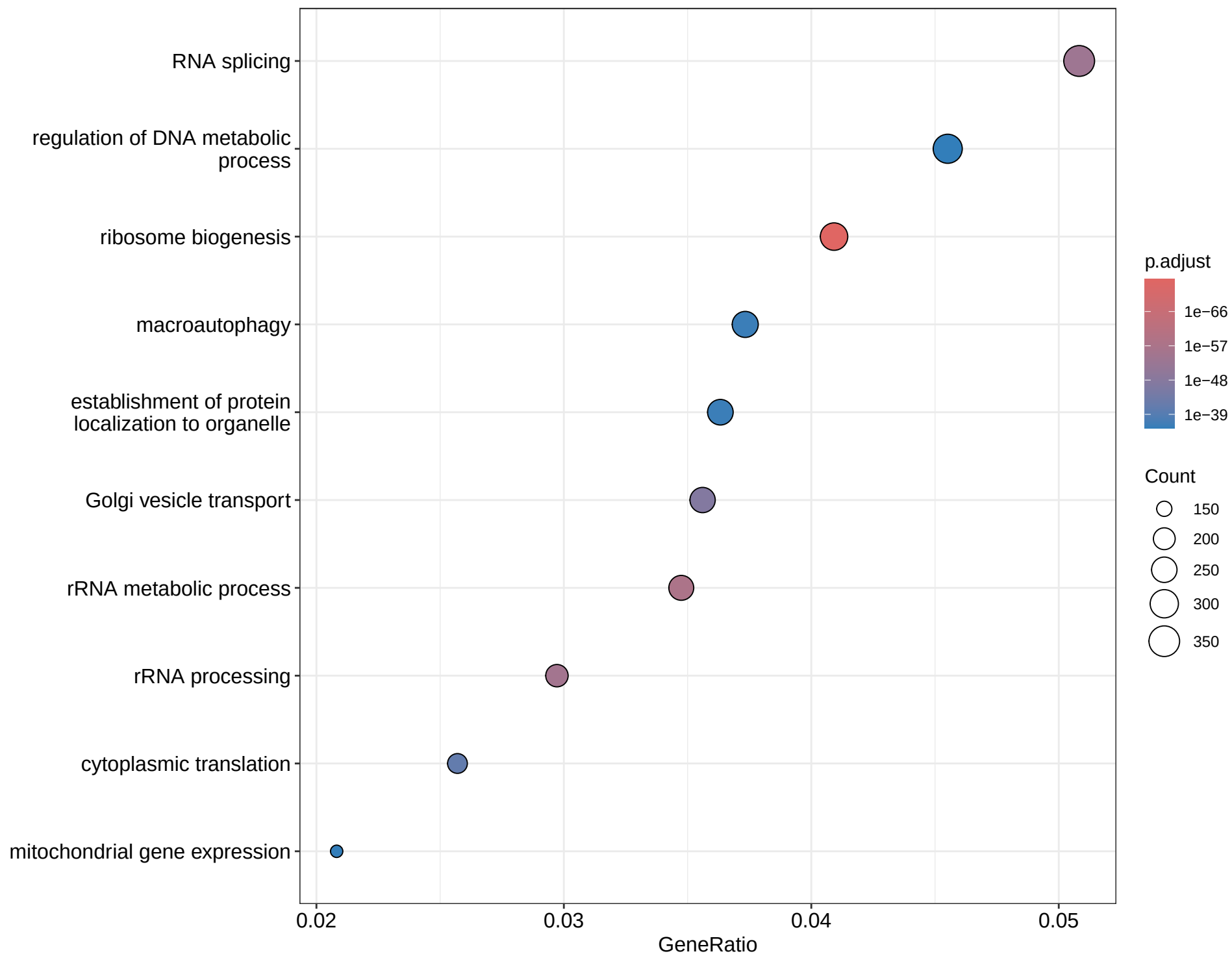
GO Enrichment: Mechanistic Stress 1
