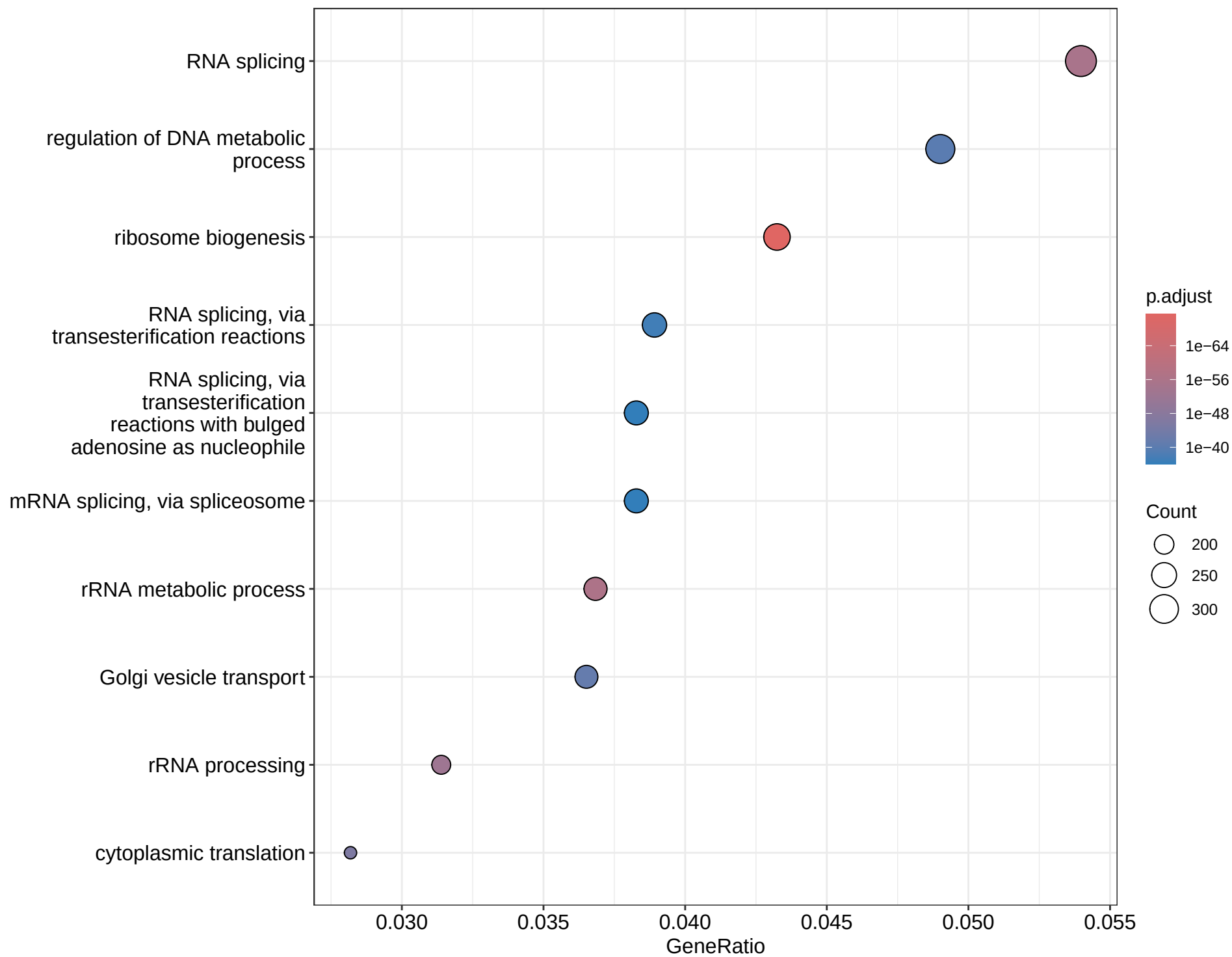
GO Enrichment: Chemical Genetic 1
