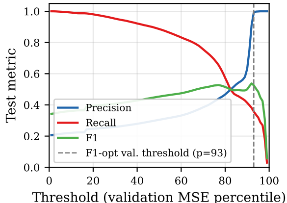
(b) Threshold sensitivity — Cross-Task FedAvg
