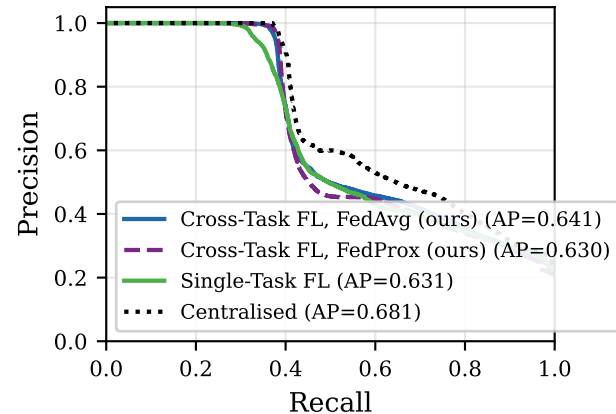
(a) Precision-Recall (LEAD test, 15 unseen)
