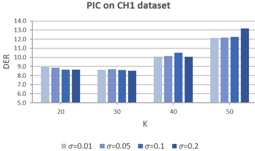
Figure 3.4: DER of CH1 dataset for different choices of number of nearest-neighbors K and scaling factor \sigma .
