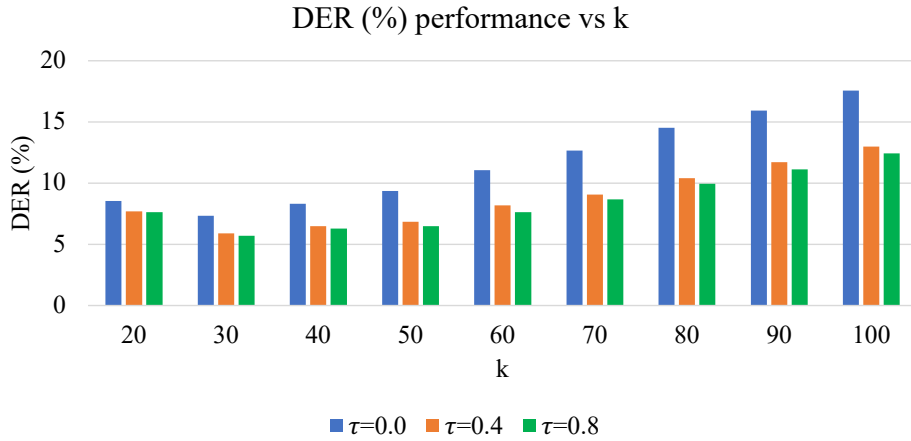
Figure 5.3: Plot comparing DER performance for k ranging from 20-100 and \tau \in \{0.0, 0.4, 0.8\} for Voxconverse dev set.
