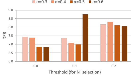
Figure 3.5: Bar plot of DER vs threshold for N^0 selection on CH1 subset of CALLHOME for different choices of \alpha parameter.
