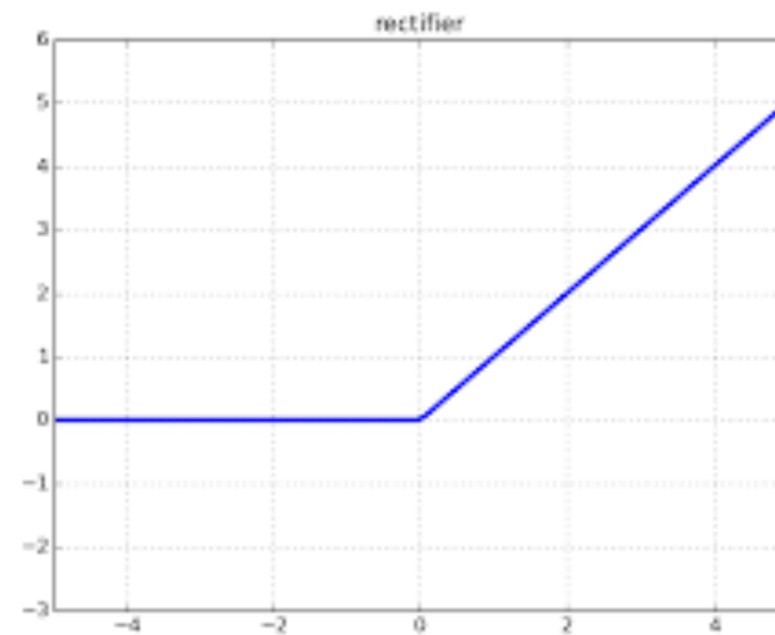
ReLu
