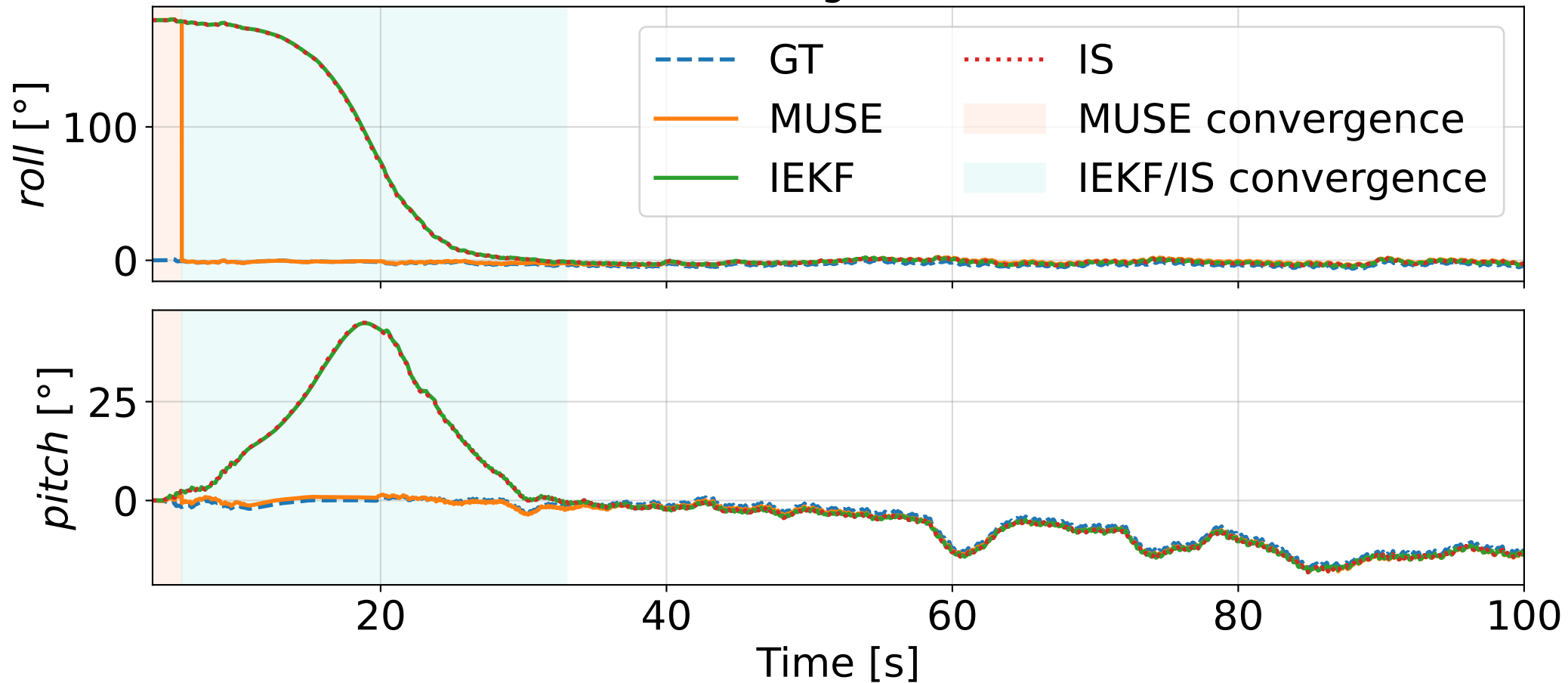
Roll and Pitch (large initial condition)
