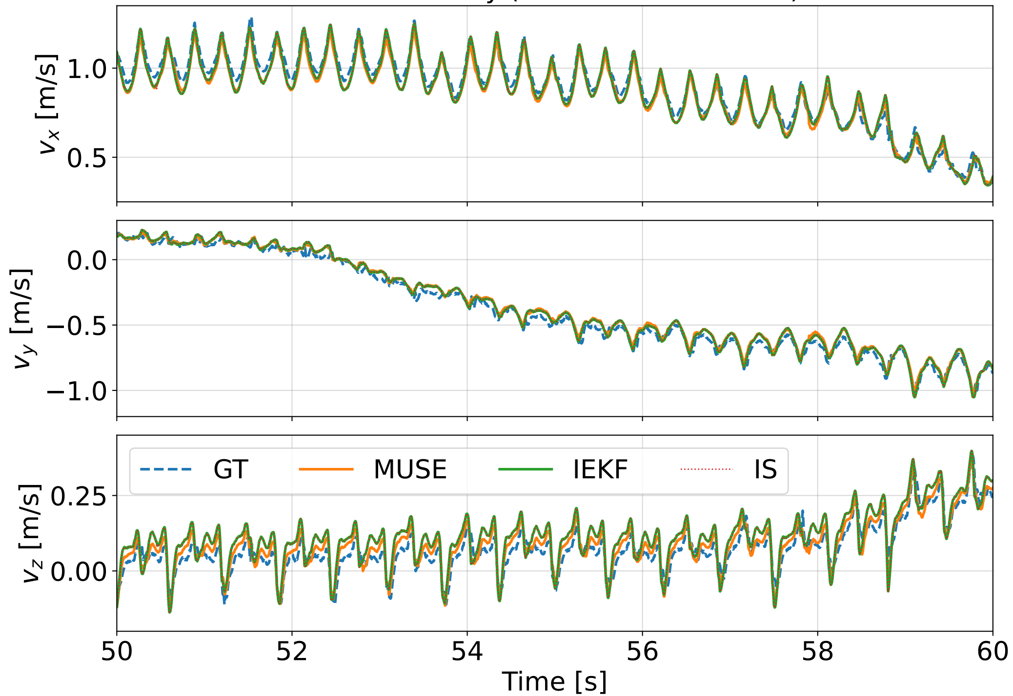
Linear Velocity (zoomed: 50.0–60.0 s)
