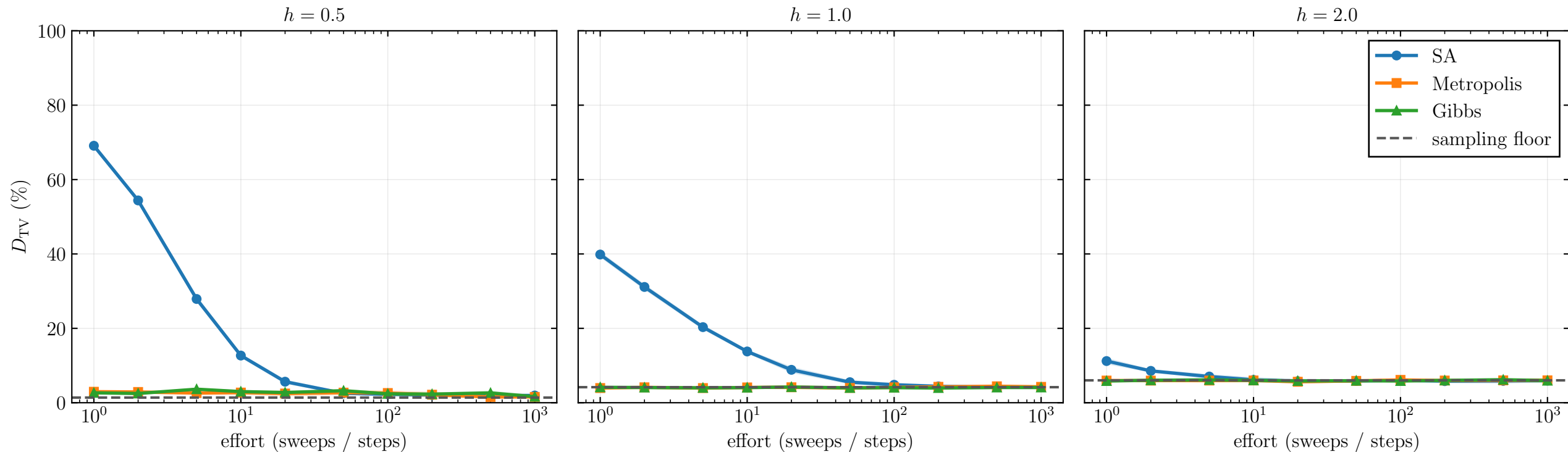
Sampling quality: SA / MH / Gibbs | TFIM 1D N = 8 n_{\text{samples}} = 10000
