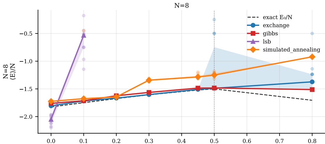
Converged \langle E \rangle / N per spin vs J_2 (heisenberg J1-J2) Median \pm IQR over seeds
