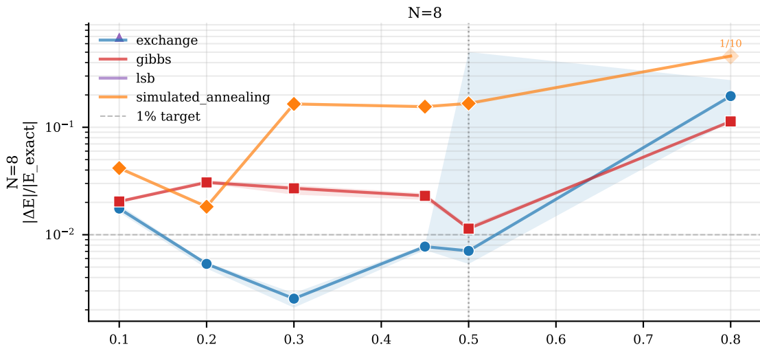
Relative energy error vs J_2 — heisenberg_j1j2_1d
