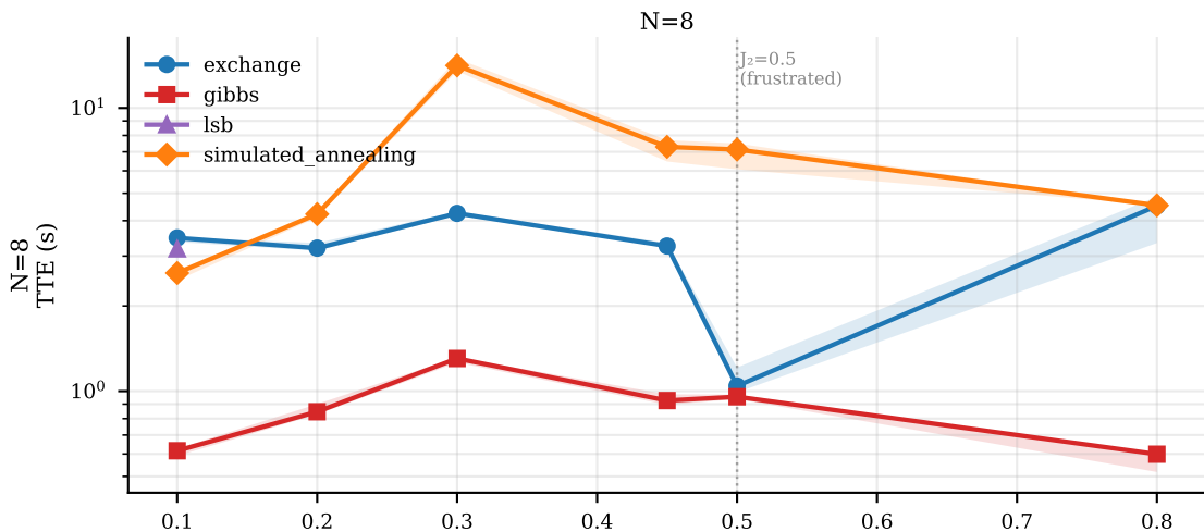
Time-to-Convergence vs J_2 (heisenberg_j1j2_1d) rolling std < 1.0\% \cdot |E_{\text{exact}}| , window=20
