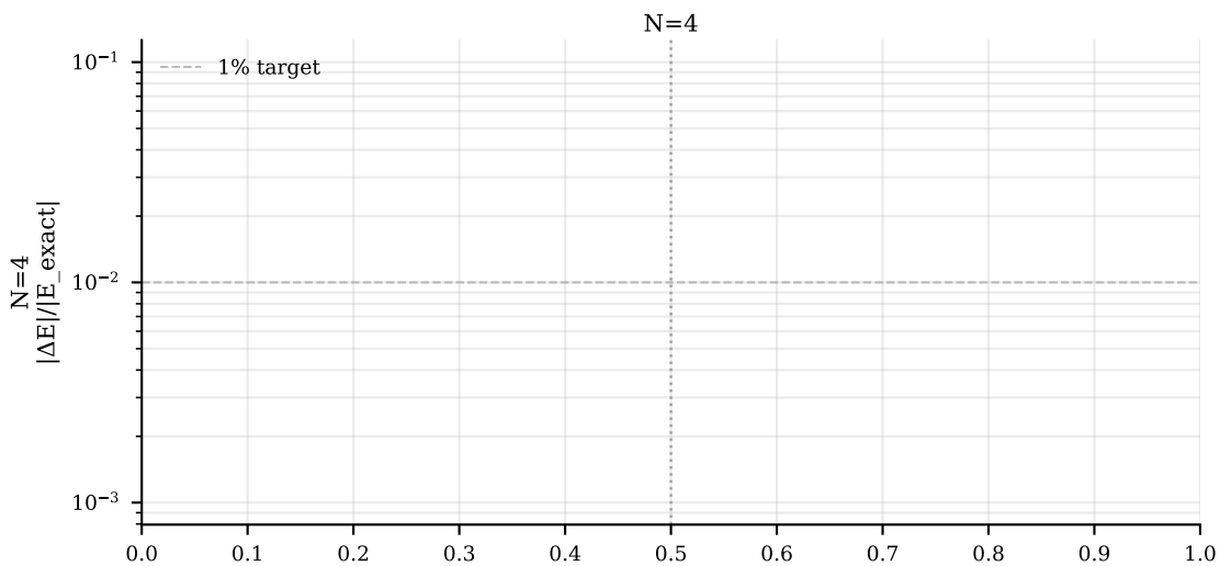
Relative energy error at convergence vs J_2 (j1j2_1d) |\Delta E|/|E_{\text{exact}}| , rolling std < 1.0%· |E_{\text{exact}}| , window=20
