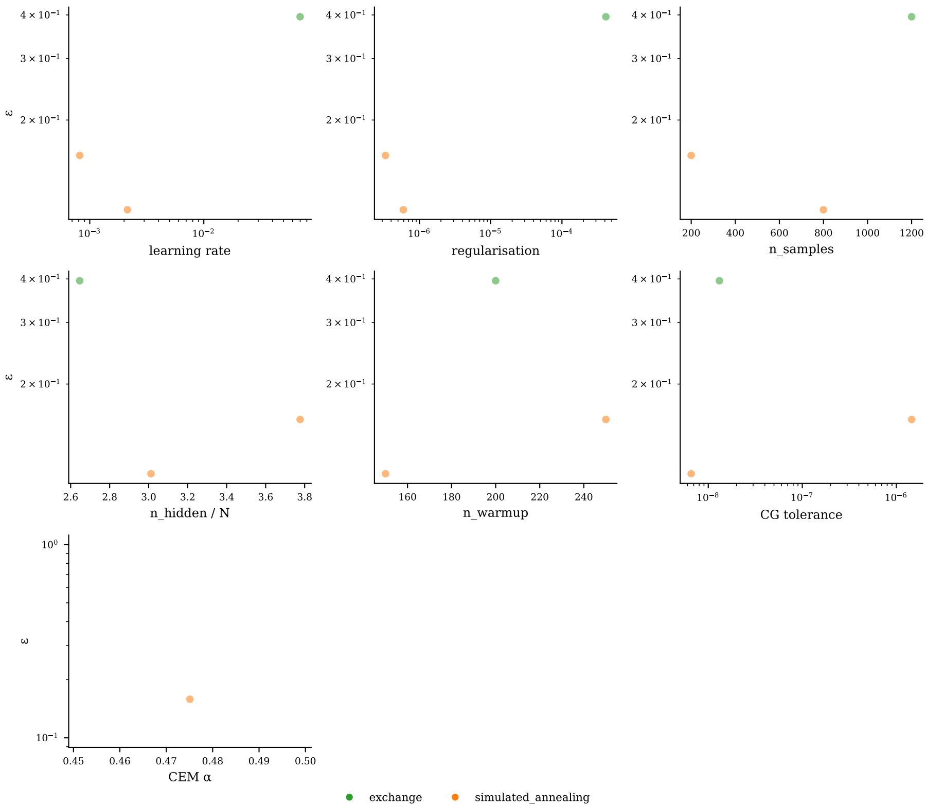
Hyperparameter sensitivity — heisenberg_j1j2_1d/heisenberg_j1j2_1d_20260528_120223/N8_J20.0
