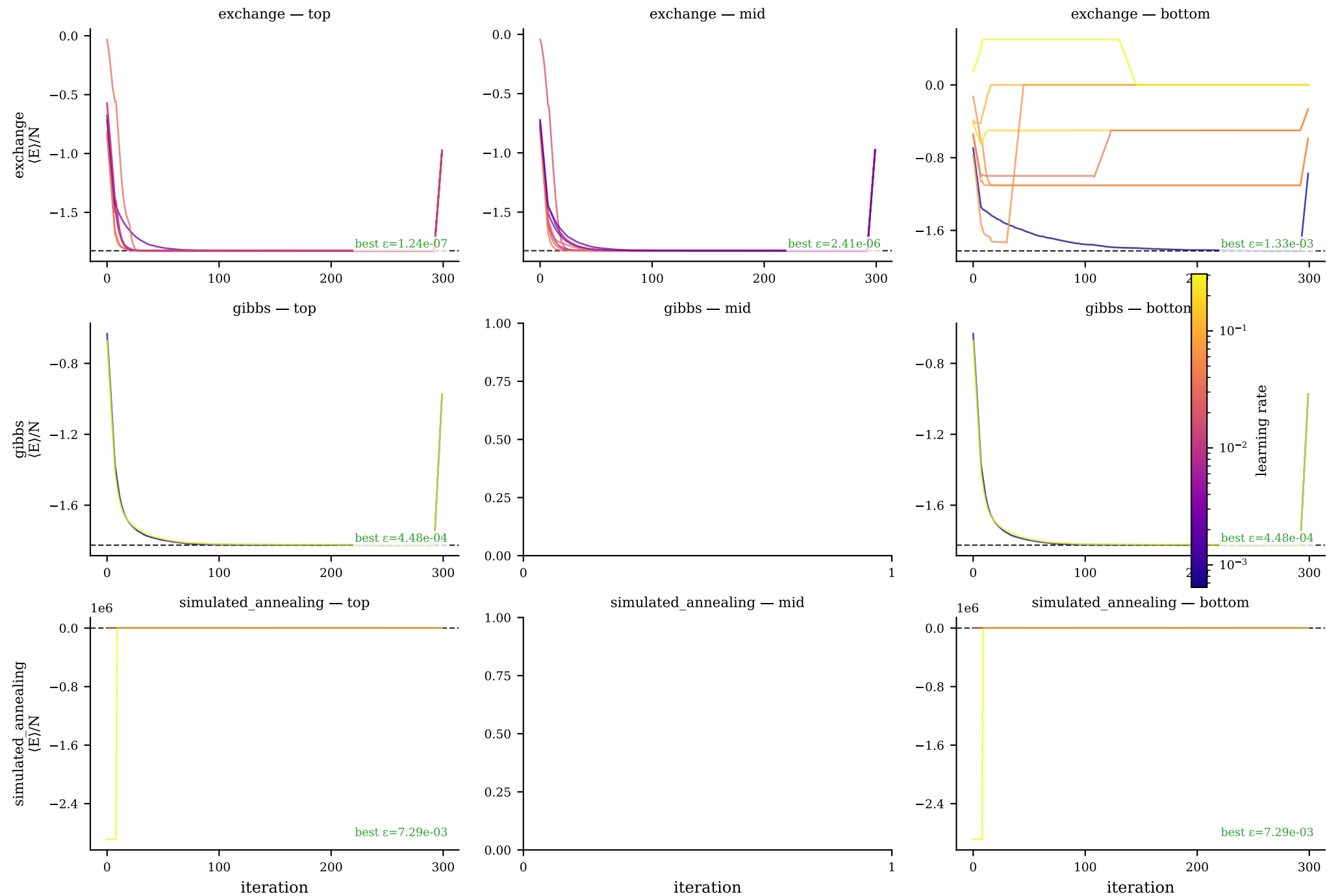
Convergence: top / mid / bottom 8 trials — heisenberg_j1j2_1d/heisenberg_j1j2_1d_20260528_120524/N8_J20.0 Colour = learning rate
