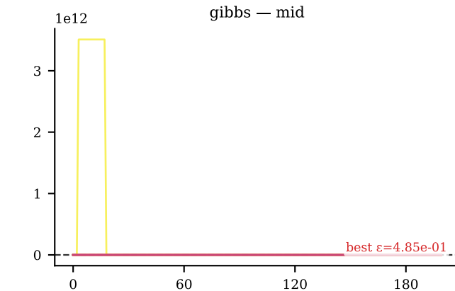
Convergence: top / mid / bottom 8 trials — heisenberg_j1j2_1d/j1j2_gibbs_lsb_v1/N8_J20.1 Colour = learning rate
