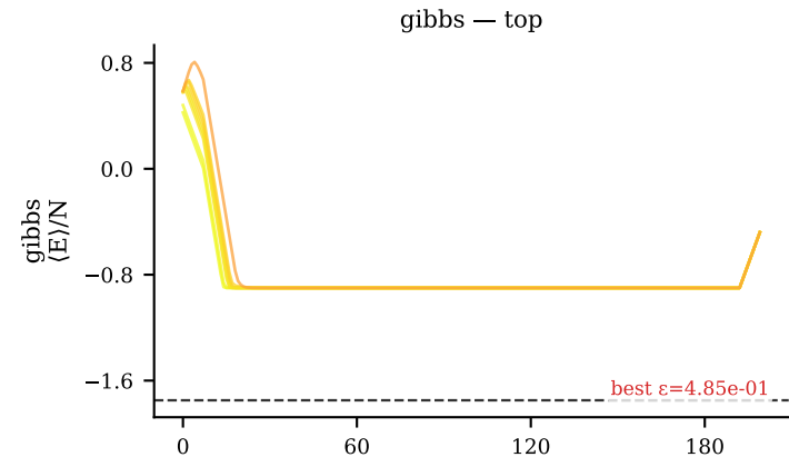
Convergence: top / mid / bottom 8 trials — heisenberg_j1j2_1d/j1j2_gibbs_lsb_v1/N8_J20.1 Colour = learning rate
