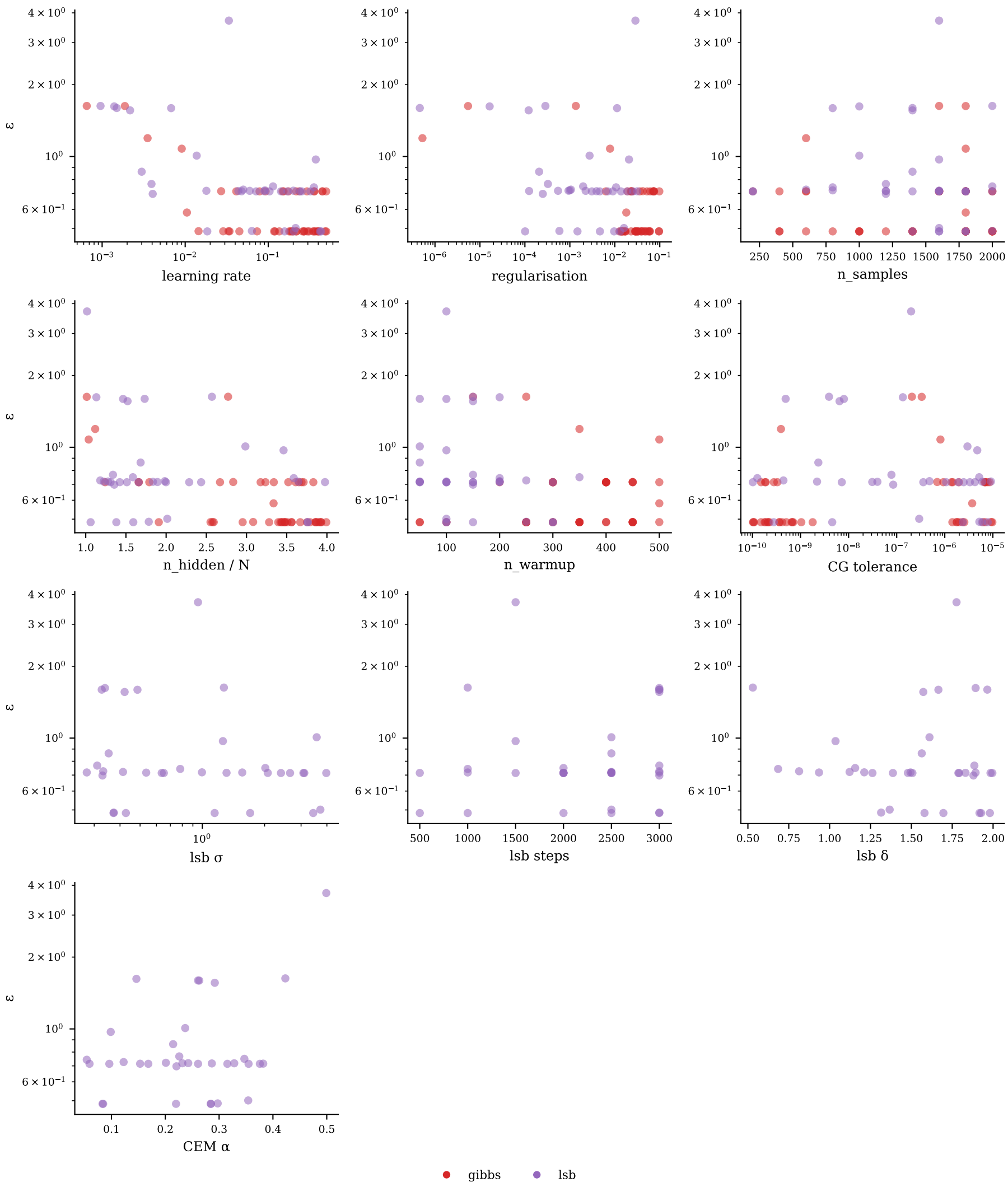
Hyperparameter sensitivity — heisenberg_j1j2_1d/j1j2_gibbs_lsb_v1/N8_J20.1
