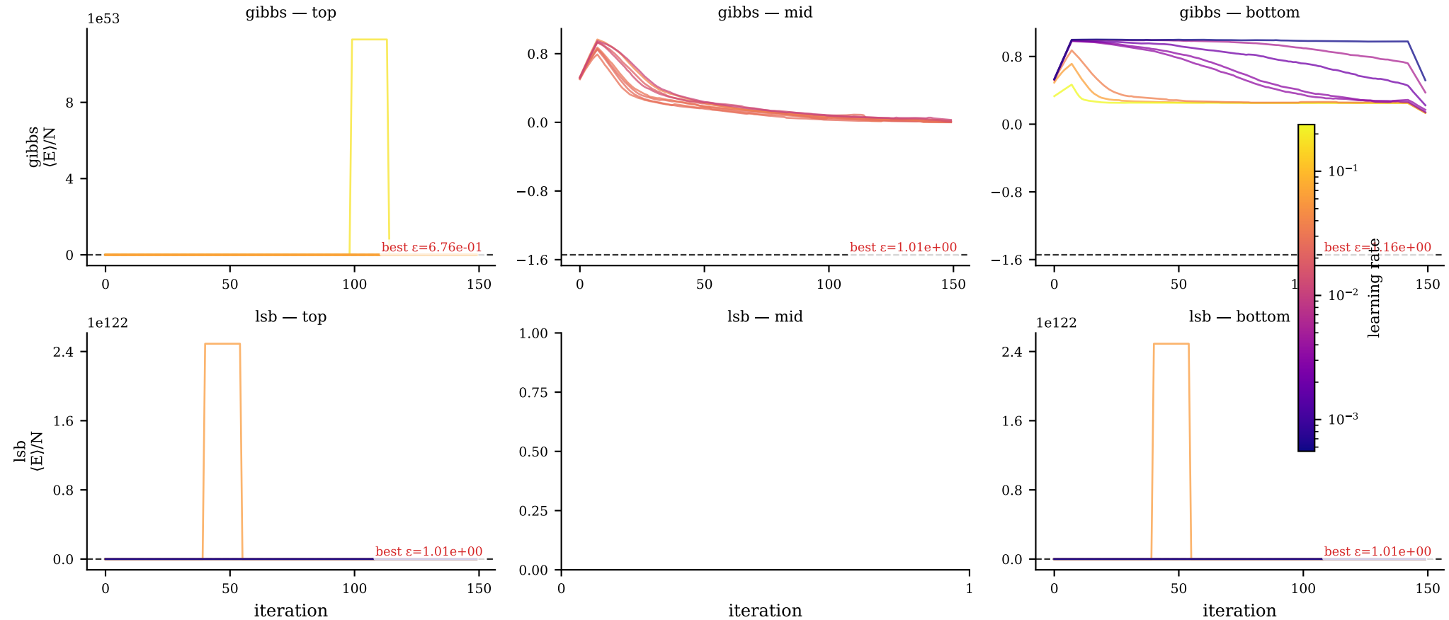
Convergence: top / mid / bottom 8 trials — heisenberg_xxz_1d/heisenberg_xxz_1d_20260527_150056/N8_delta0.5 Colour = learning rate
