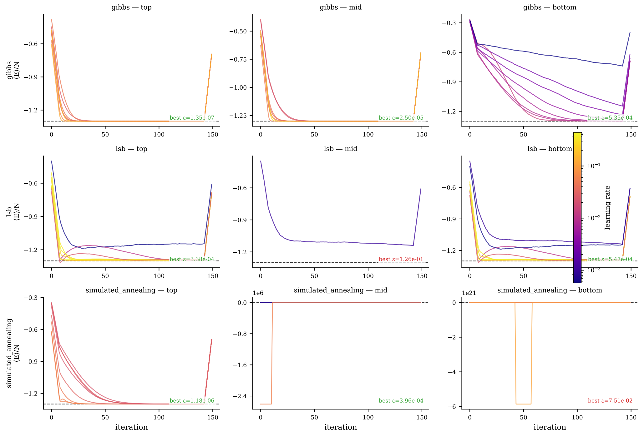
Convergence: top / mid / bottom 8 trials — j1j2_1d/j1j2_1d_20260527_152843/N8_J20.25 Colour = learning rate
