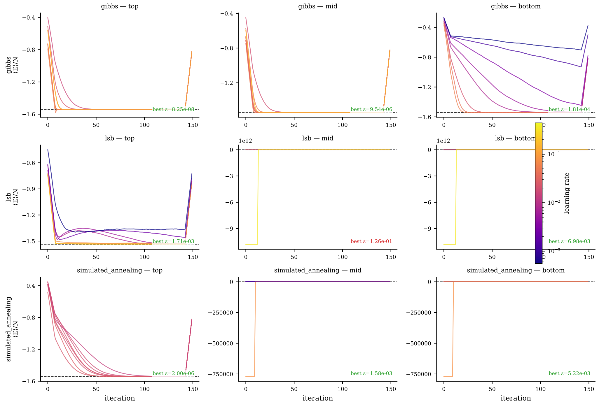
Convergence: top / mid / bottom 8 trials — j1j2_1d/j1j2_1d_20260527_152843/N8_J20.5 Colour = learning rate
