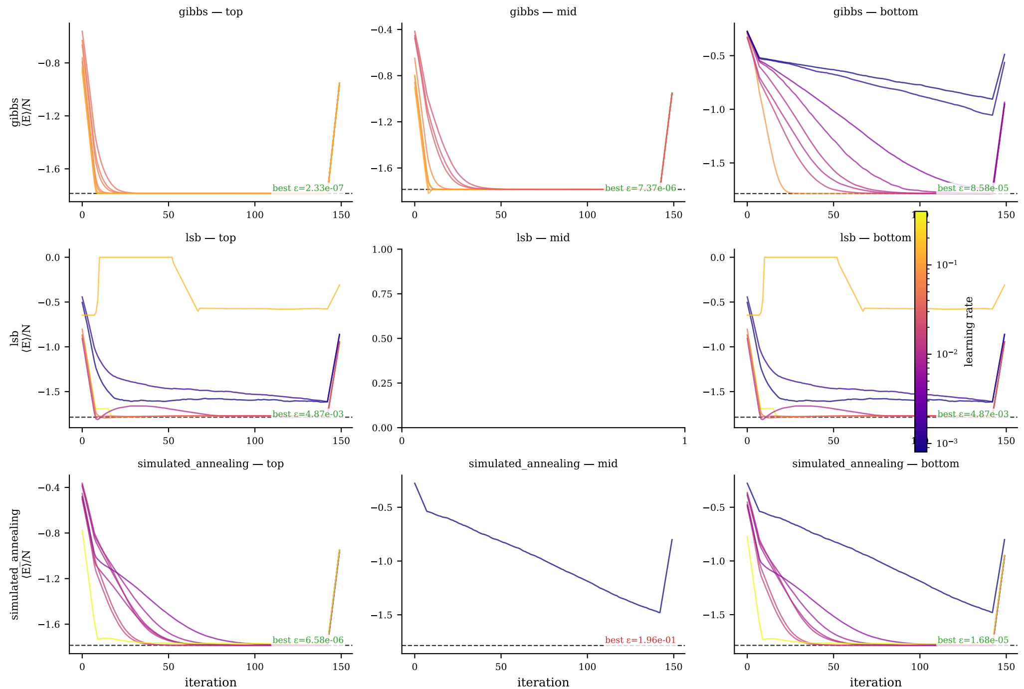
Convergence: top / mid / bottom 8 trials — j1j2_1d/j1j2_1d_20260527_152843/N8_J20.75 Colour = learning rate
