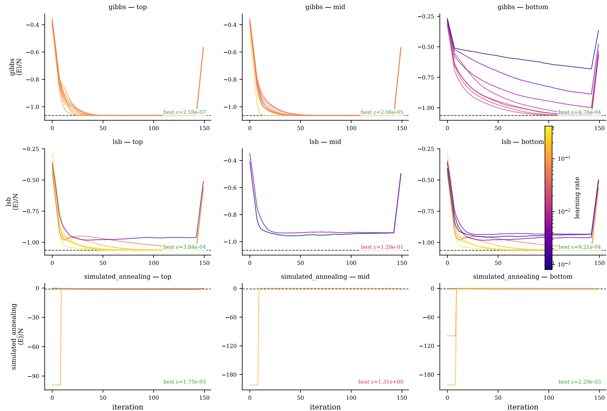
Convergence: top / mid / bottom 8 trials — j1j2_1d/j1j2_1d_20260527_170753/N12_J20.0 Colour = learning rate
