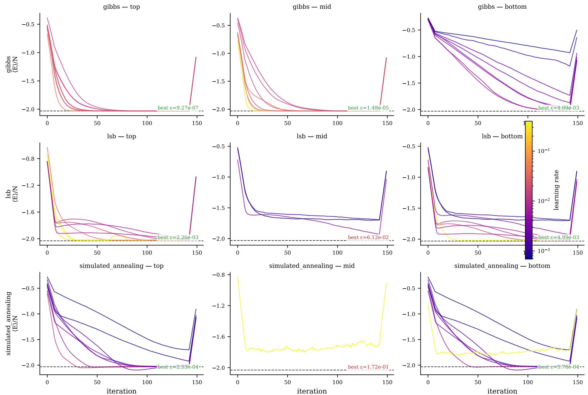
Convergence: top / mid / bottom 8 trials — j1j2_1d/j1j2_1d_20260527_170753/N16_J21.0 Colour = learning rate
