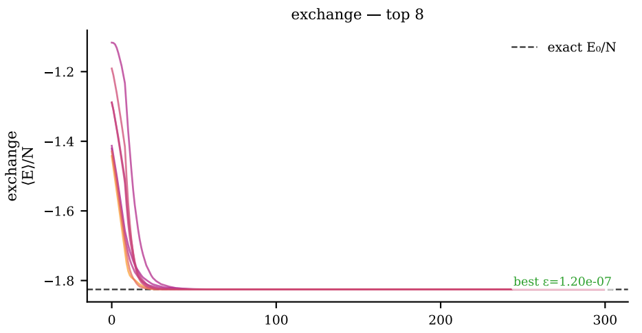
Best 8 convergence curves — heisenberg_j1j2_1d/heisenberg_j1j2_1d_20260528_120524/N8_J20.0 ( |E/N| \leq 10.0 ) Colour = learning rate
