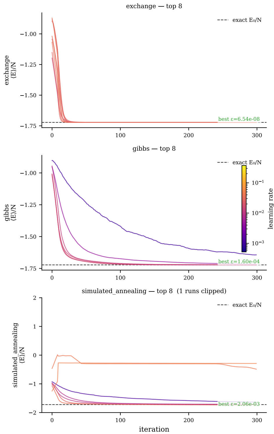
Best 8 convergence curves — heisenberg_j1j2_1d/heisenberg_j1j2_1d_20260528_124115/N12_J20.1 ( |E/N| \leq 10.0 ) Colour = learning rate
