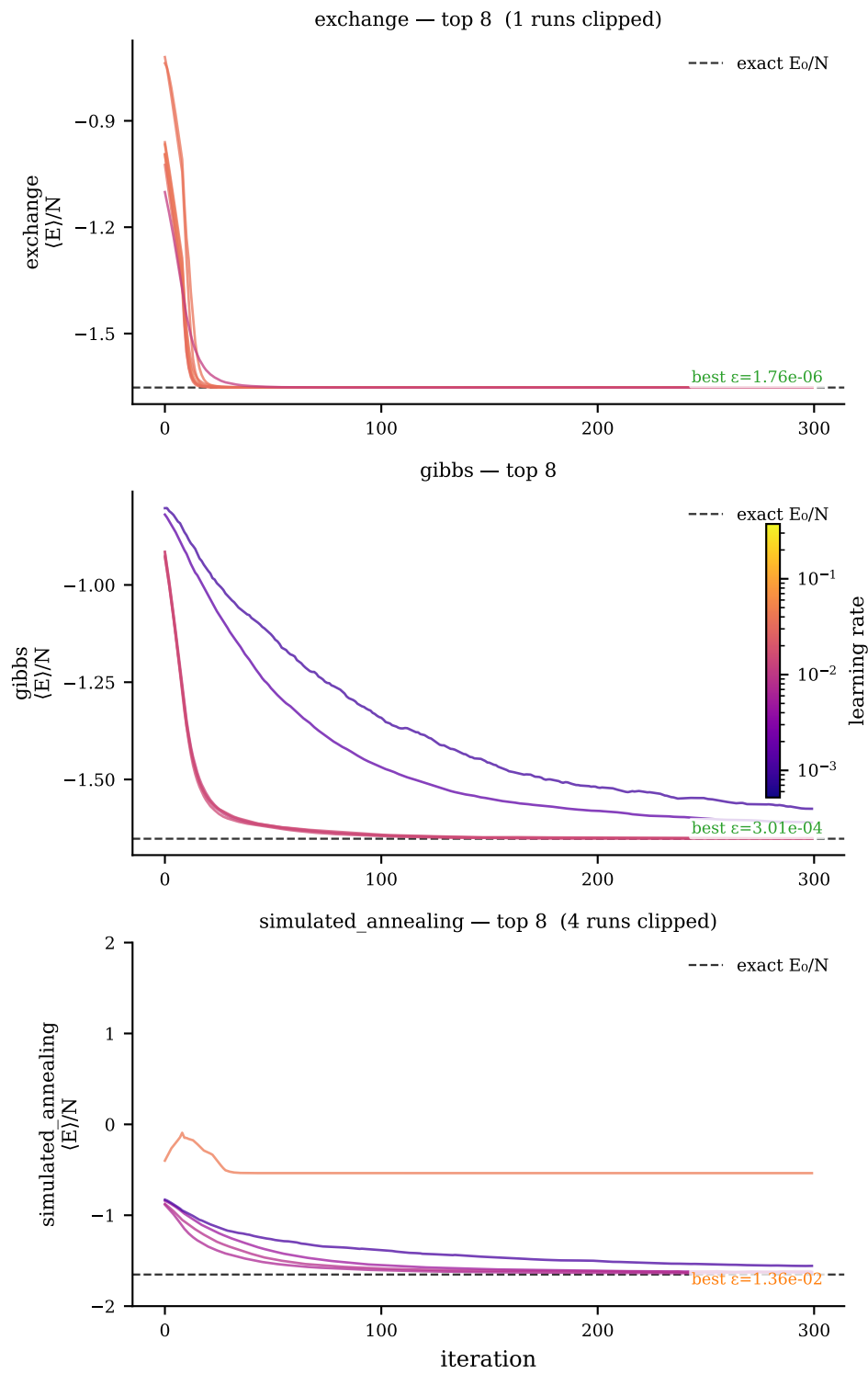
Best 8 convergence curves — heisenberg_j1j2_1d/heisenberg_j1j2_1d_20260528_124115/N12_J20.2 ( |E/N| \leq 10.0 ) Colour = learning rate
