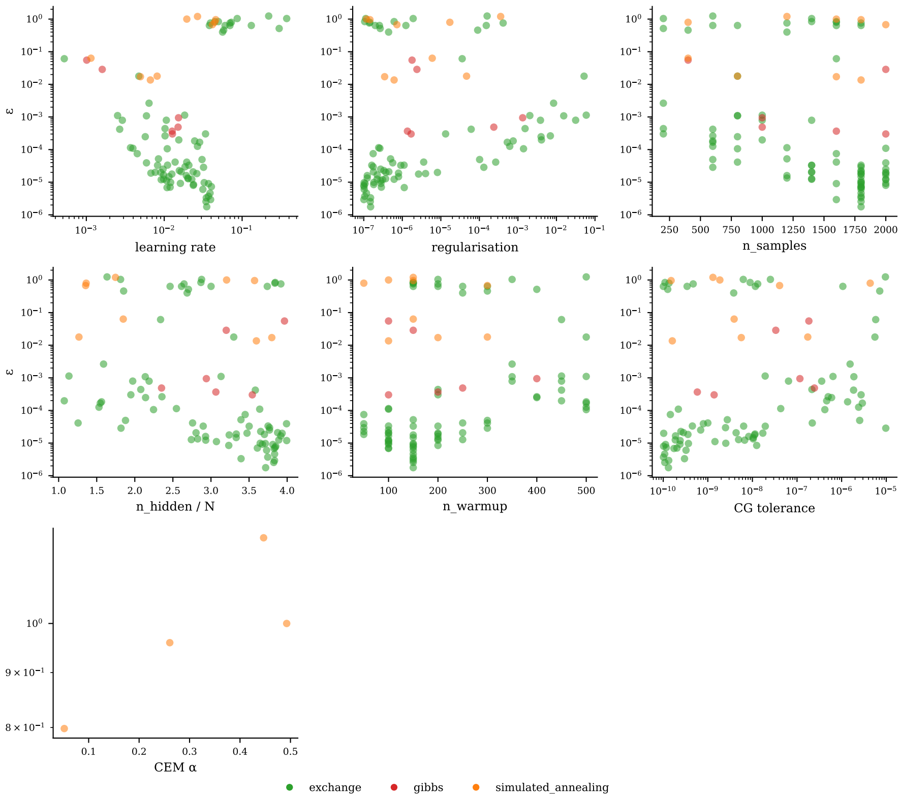
Hyperparameter sensitivity — heisenberg_1j2_1d/heisenberg_1j2_1d_20260528_124115/N12_J20.2
