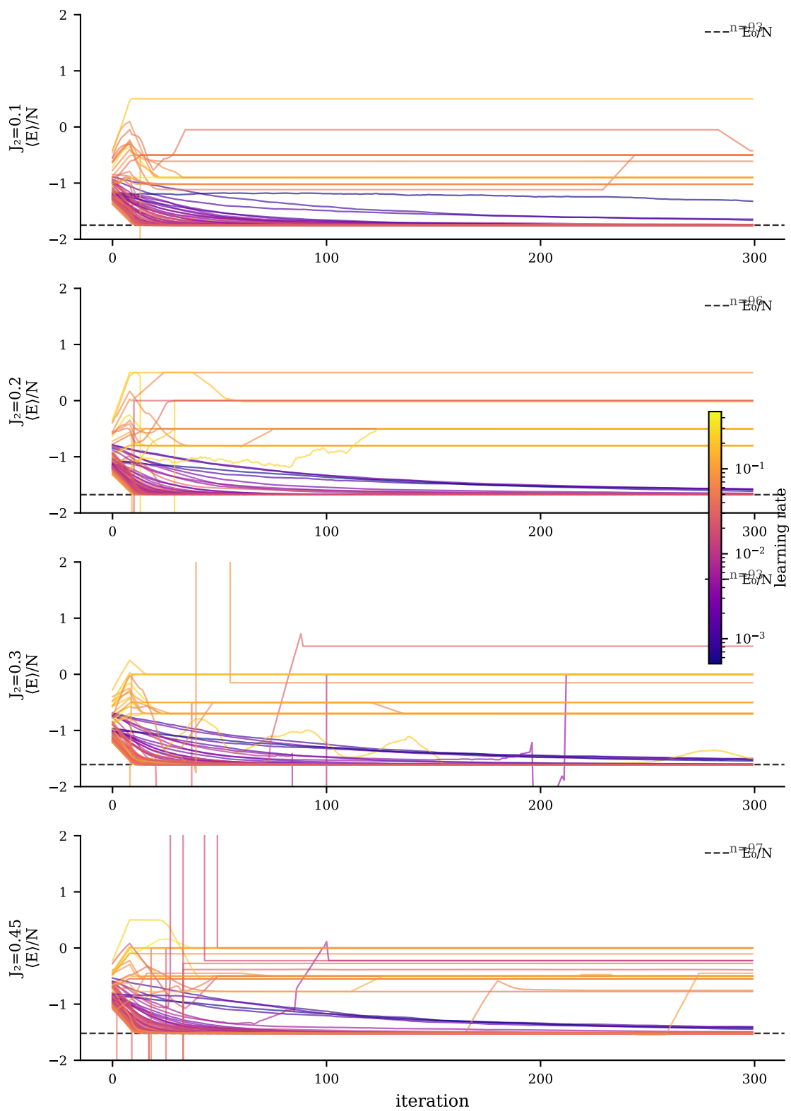
Convergence per J_2 — heisenberg_j1j2_1d/heisenberg_j1j2_1d_20260528_124115/N8 Each line = one trial · colour = learning rate
