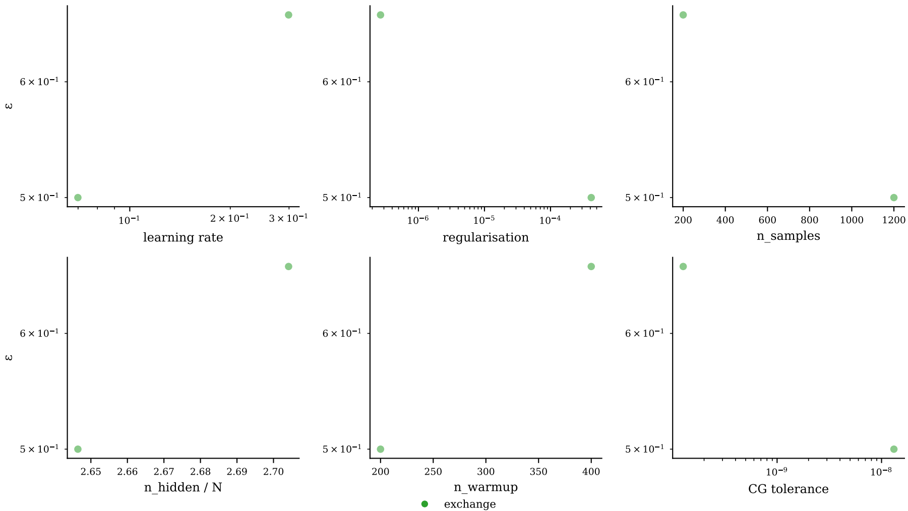
Hyperparameter sensitivity — heisenberg_j1j2_1d/heisenberg_j1j2_1d_20260529_102104/N8_J20.5
