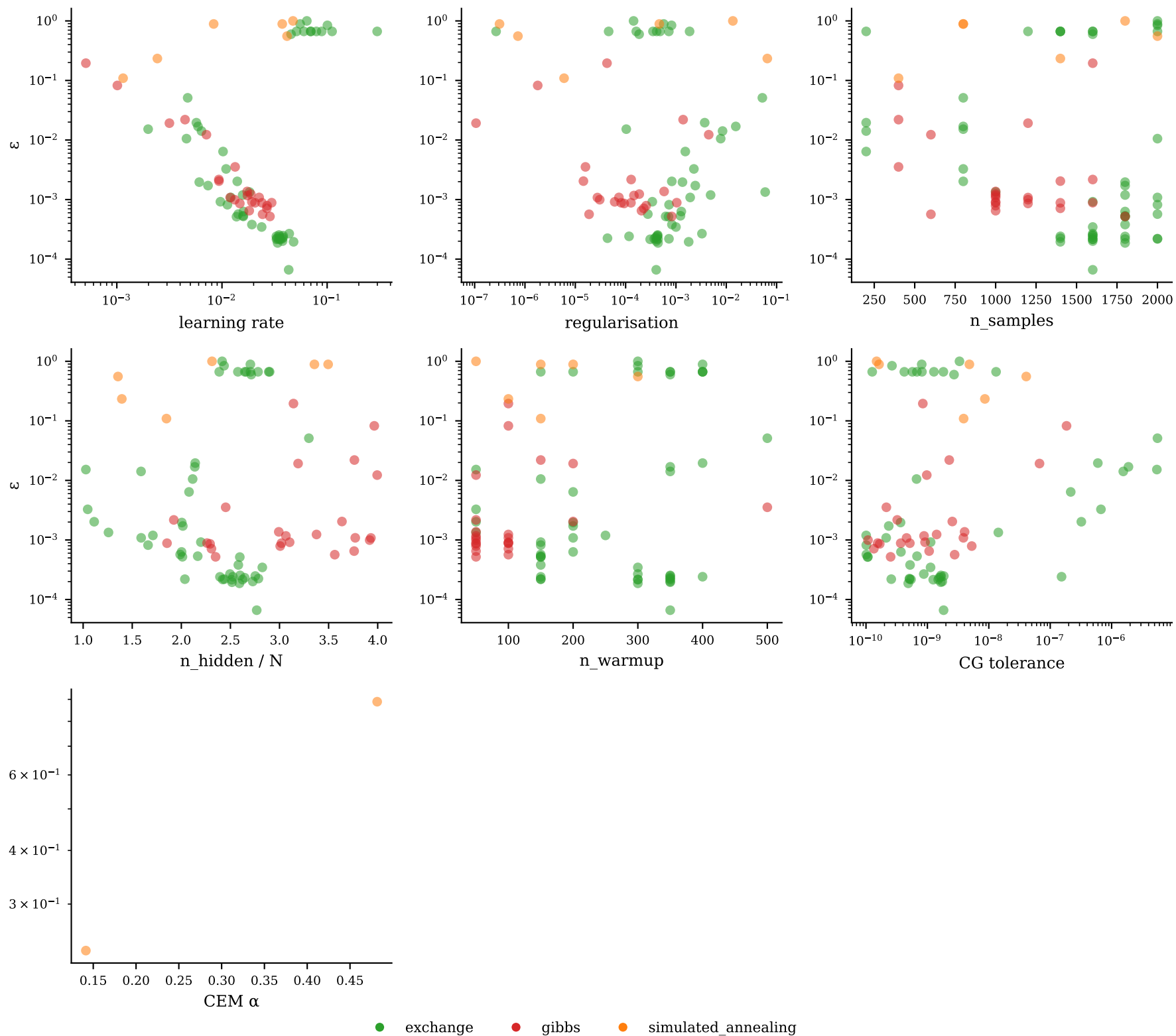
Hyperparameter sensitivity — heisenberg_1j2_1d/heisenberg_1j2_1d_20260529_102239/N12_J20.5
