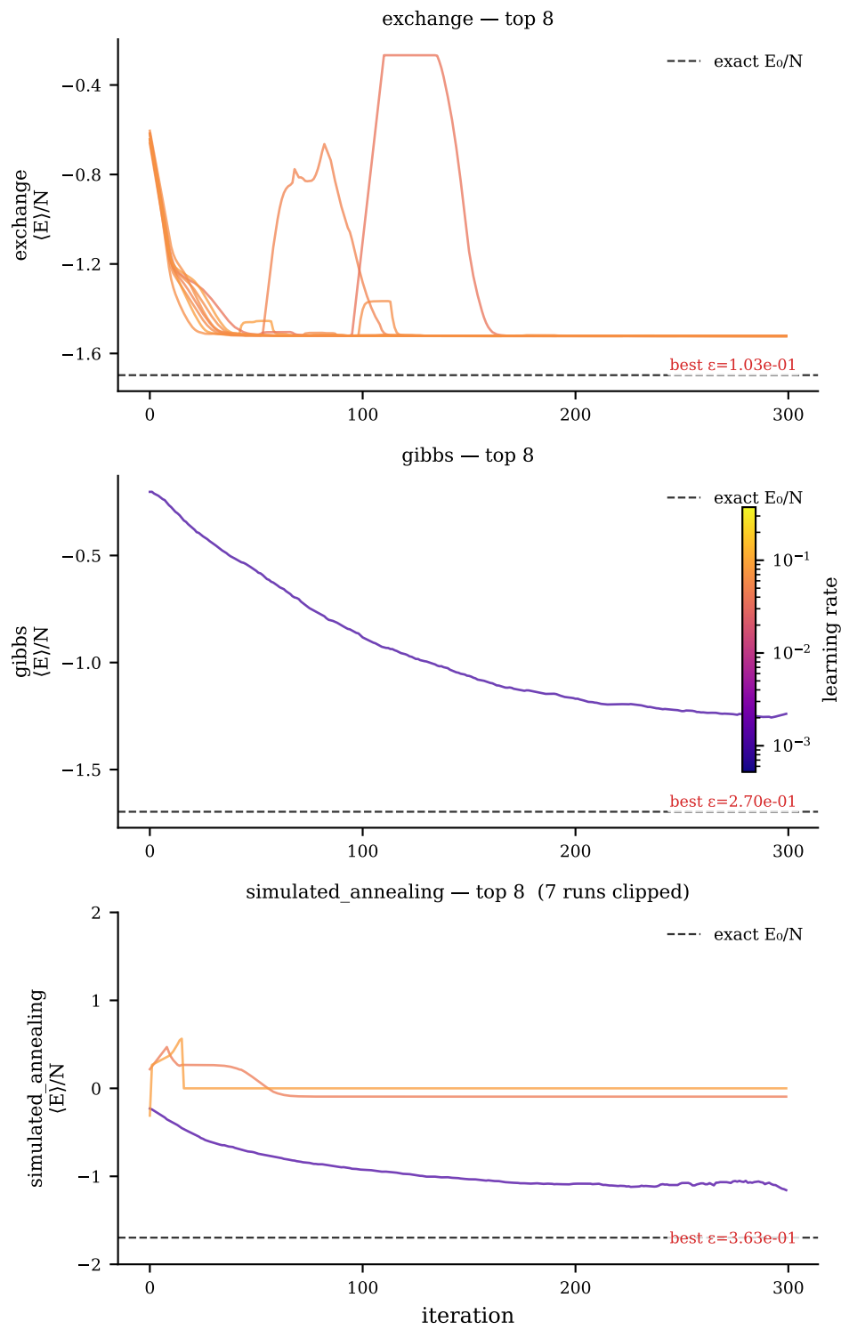
Best 8 convergence curves — heisenberg_j1j2_1d/heisenberg_j1j2_1d_20260529_102239/N12_J20.8 ( |E/N| \leq 10.0 ) Colour = learning rate
