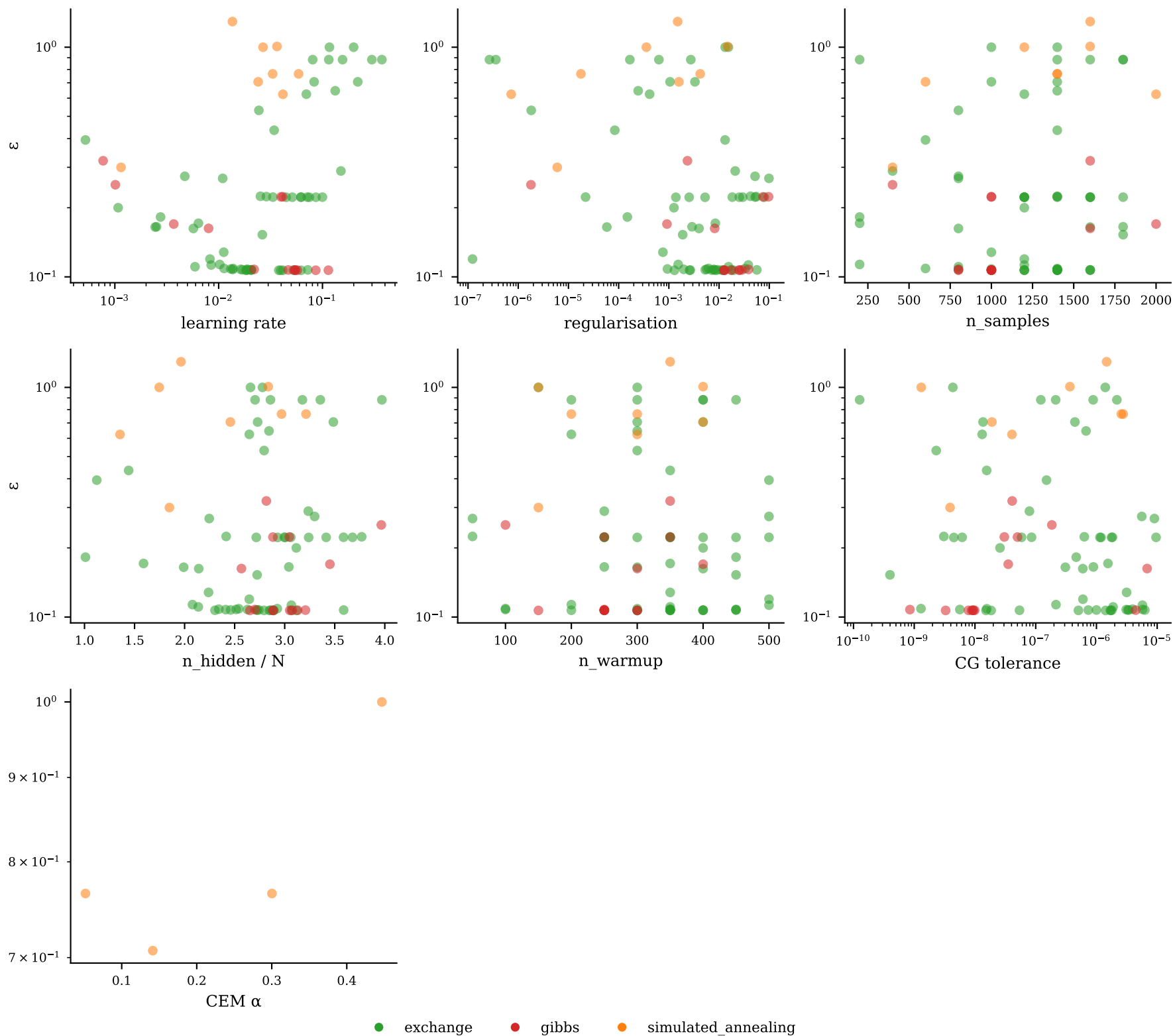
Hyperparameter sensitivity — heisenberg_j1j2_1d/heisenberg_j1j2_1d_20260529_102239/N8_J20.8
