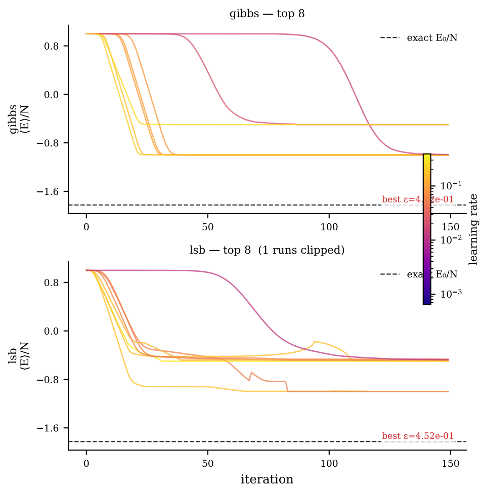
Best 8 convergence curves — heisenberg_xxz_1d/heisenberg_xxz_1d_20260527_150056/N8_delta1.0 ( |E/N| \leq 10.0 ) Colour = learning rate
