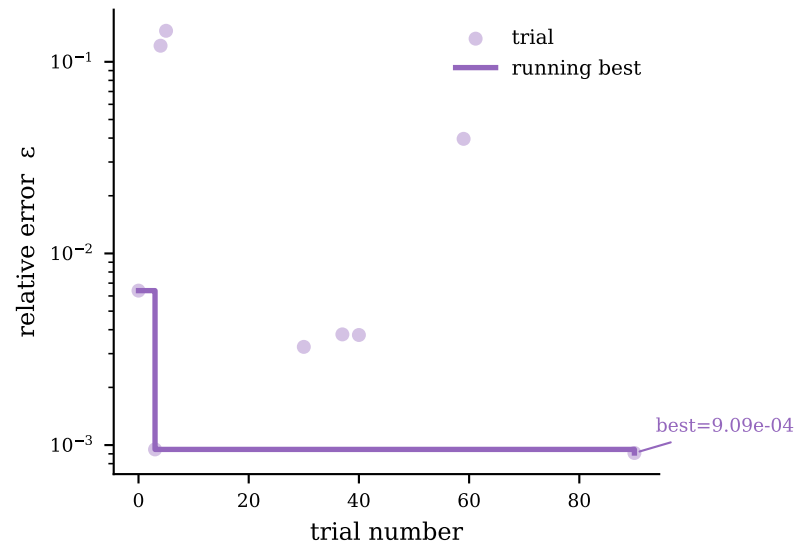
lsb (9 trials)
