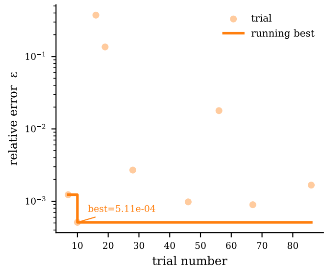
simulated_annealing (9 trials)
