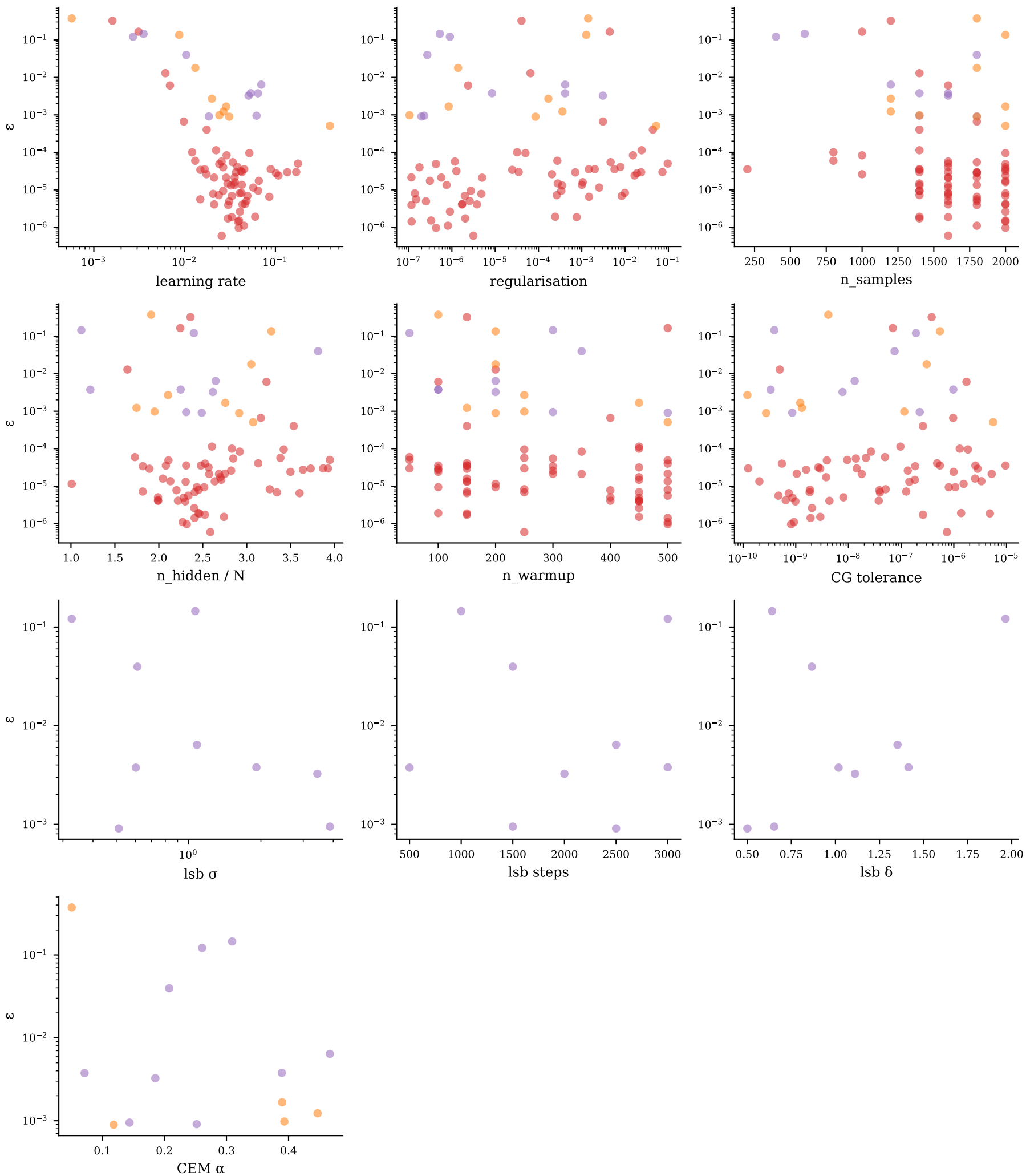
Hyperparameter sensitivity — j1j2_1d/j1j2_1d_20260527_170753/N12_J20.25
